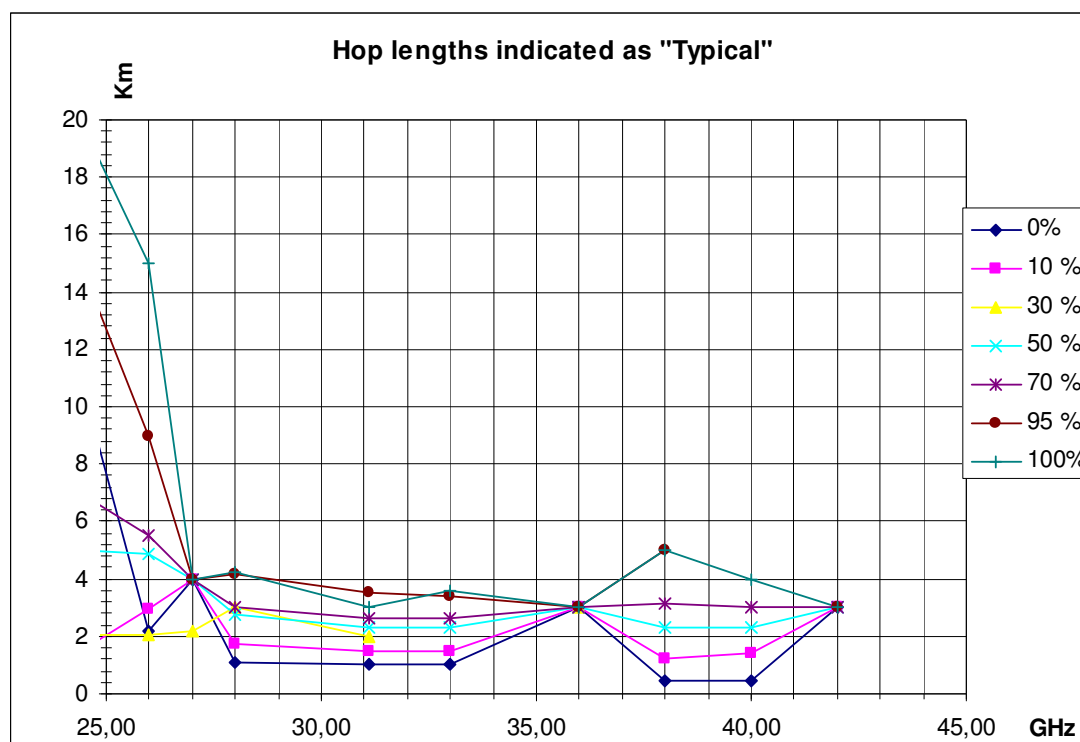
Figure 30: Typical hop length for frequency bands from 25 to 45 GHz
